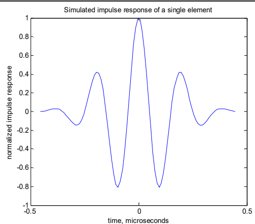
Fig. (a2) Element impulse response
