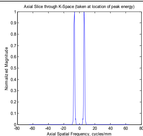
Fig. (i2) K space axial slice
