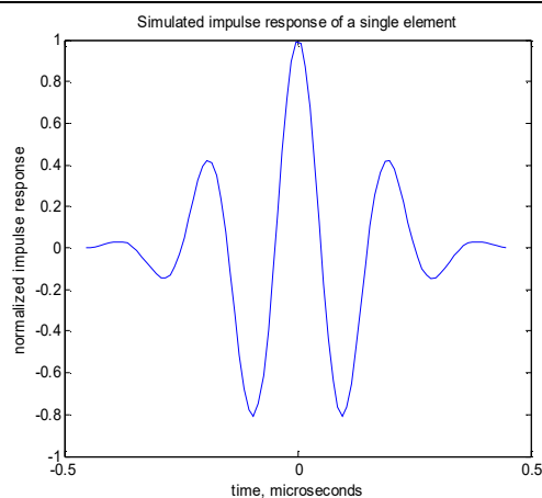
Fig. (a1) Element impulse response
