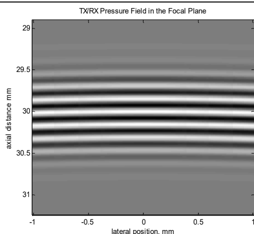
Fig. (e1) TX/RX Field image
