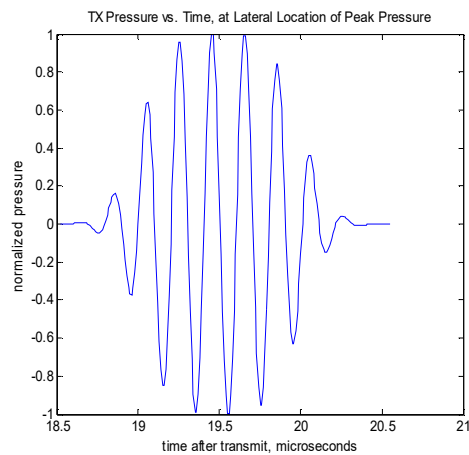
Fig. (c1) TX Axial waveform
