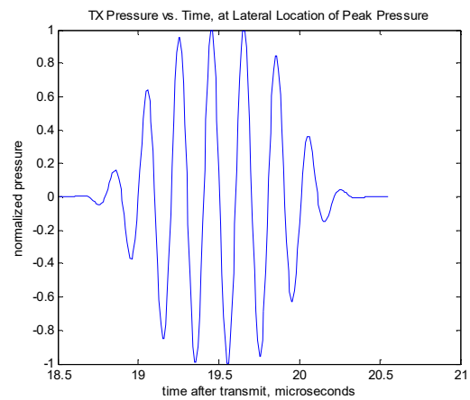
Fig. (c2) TX Axial waveform
