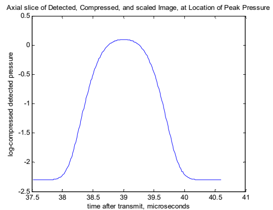
Fig. (I2) Detected image axial slice
