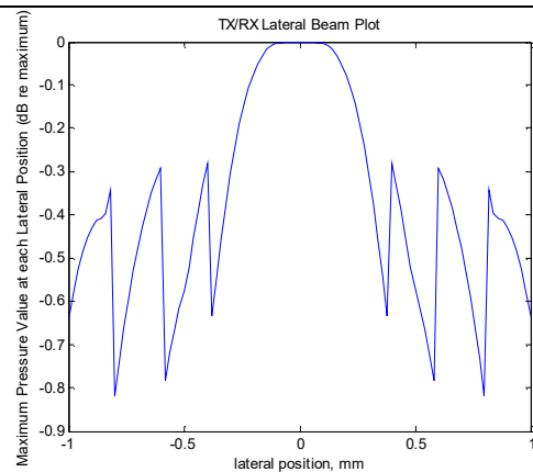
Fig. (g1) TX/RX Lateral beam-plot
