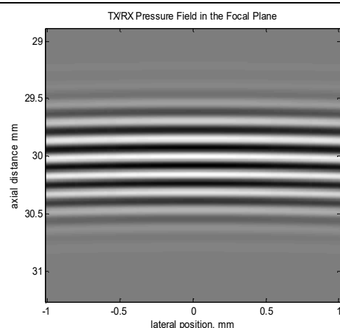
Fig. (e2) TX/RX Field image
