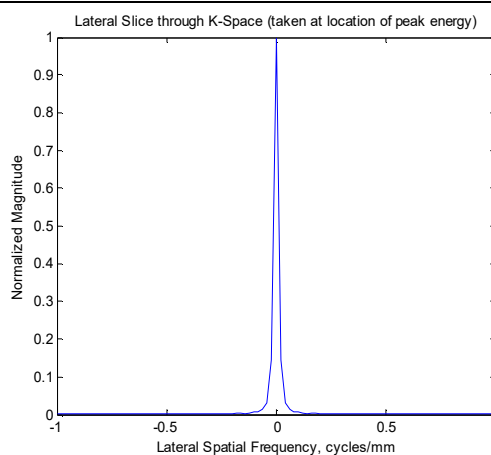
Fig. (j2) K space lateral slice
