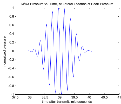
Fig. (f2) TX/RX Axial waveform
