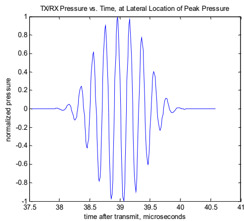
Fig. (f1) TX/RX Axial waveform
