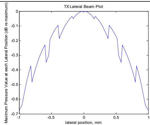
Fig. (d2) TX Lateral beam-plot
