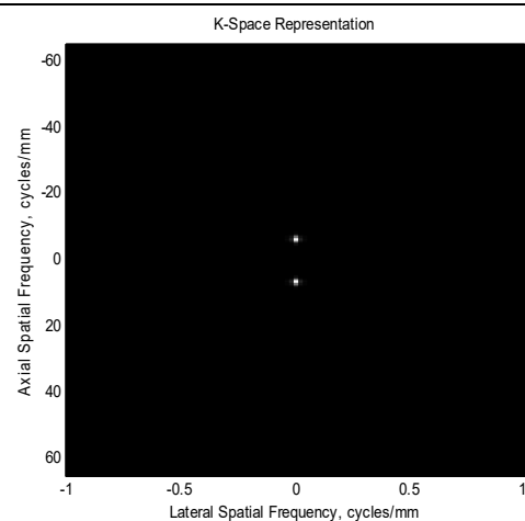
Fig. (h2) K space TX/RX Field image
