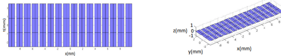
Fig. (1) Design format of linear array transducer (Height=5mm, Width=0.25mm, Kerf=0.02mm)
