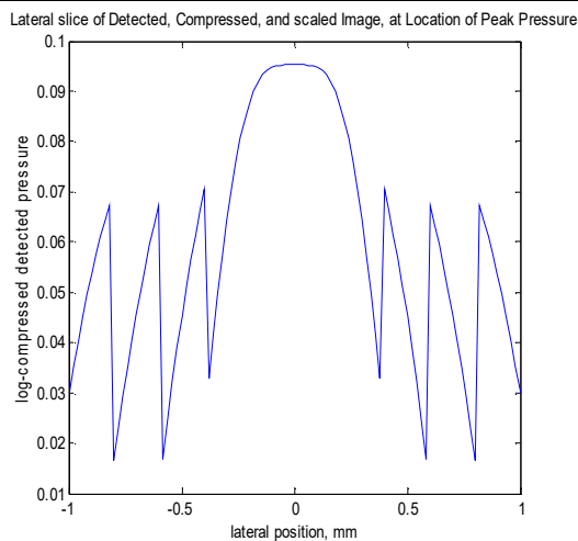
Fig.(m1) Detected image lateral slice
