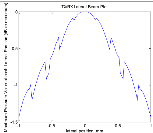
Fig. (g2) TX/RX Lateral beam-plot
