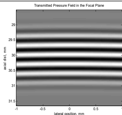
Fig.(b1) TX Field image
