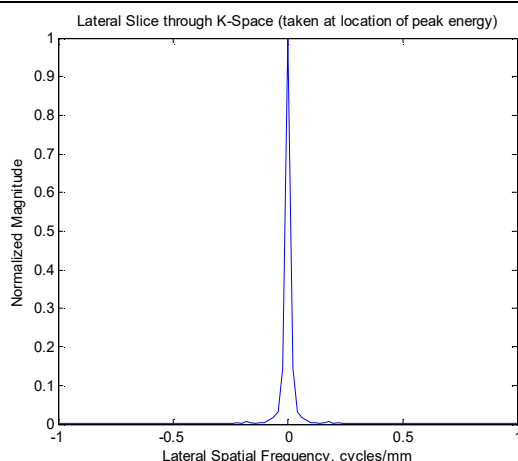
Fig. (j1) K space lateral slice
