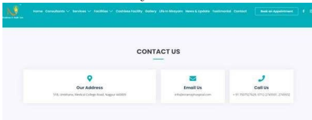
Fig 5: Contact US
