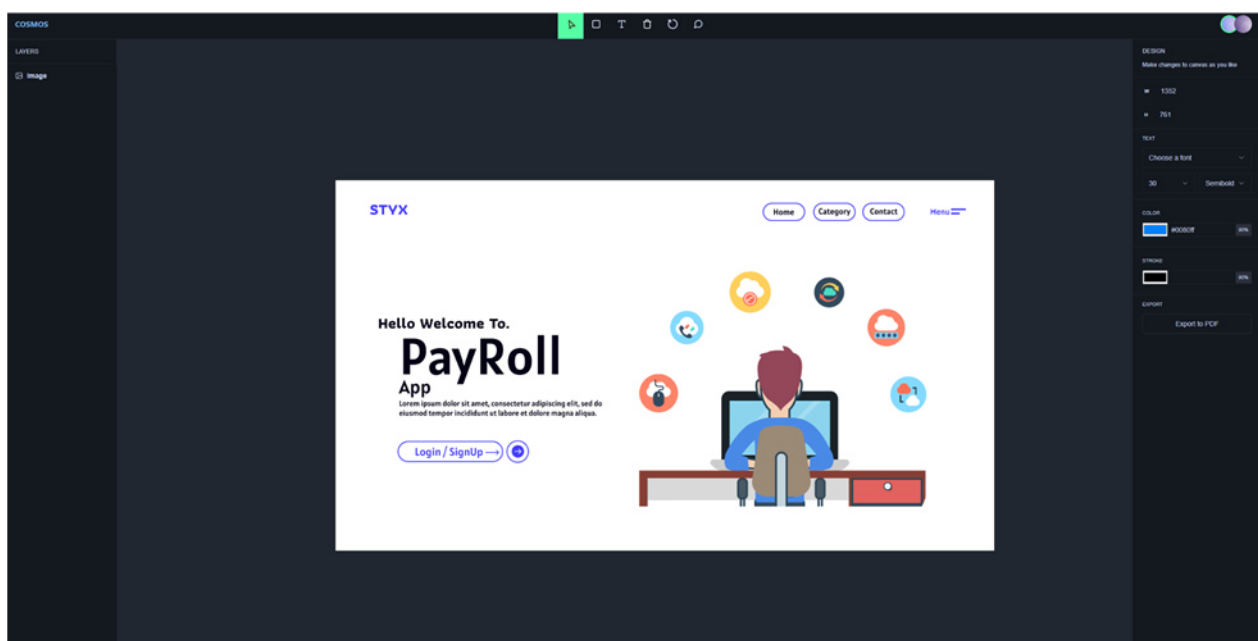
Fig 2: Use Case
