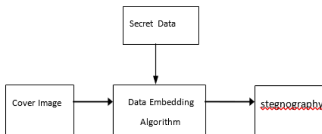
Fig 1 : Steganography Diagram
