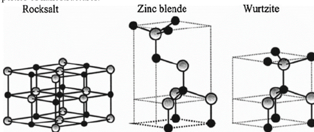
Figure 2. Various structural phases of ZnO crystal.
