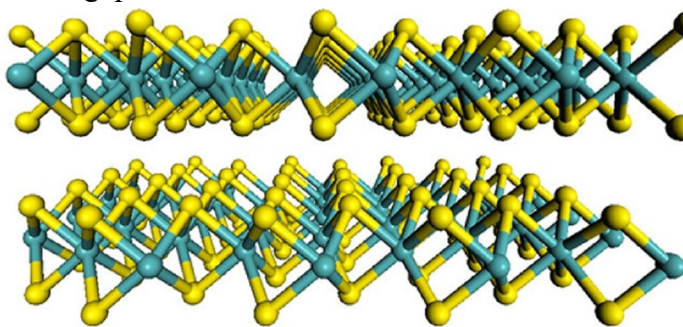
Figure 3. Molybdenum disulfide.
